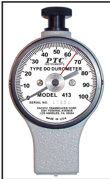
Model 413 ASTM Type DO Durometer for dense textile windings, medium-hard printing rollers, and similar materials
