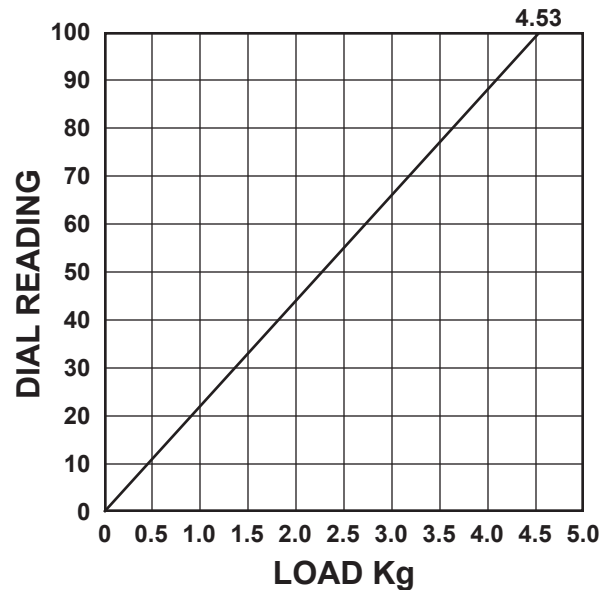
Force curve for Model 413 (ASTM D2240 Type DO)
