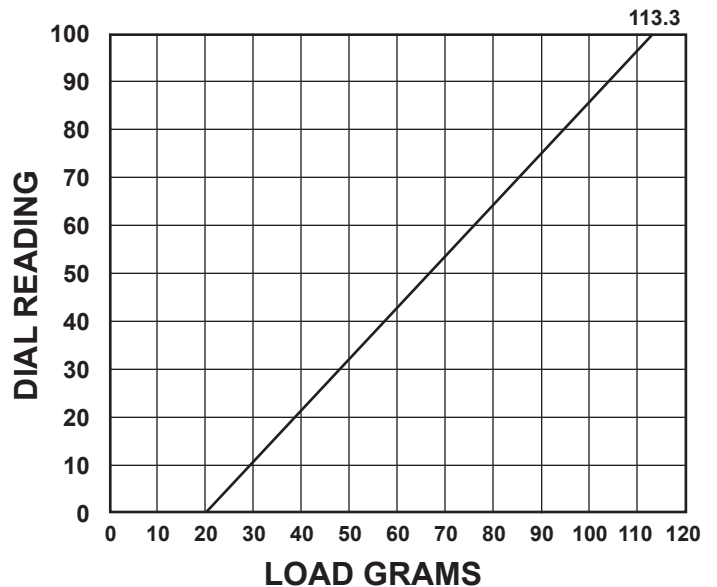
Force curve for Model 412 ASTM Type OOO
