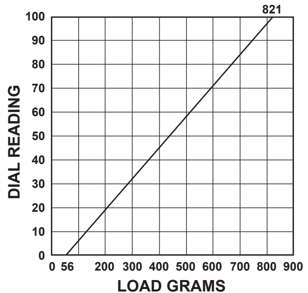
Force curve for Model 408 (ASTM D2240 Type A)
