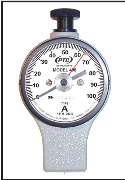
Model 408 ASTM Type A Durometer for rubber, rubber-like materials, and soft plastics
