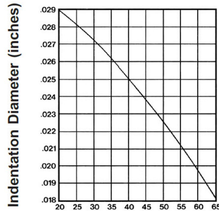
Equivalent Rockwell C Scale
