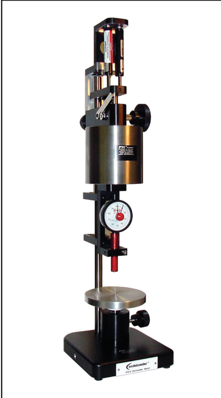
Model 474-2 ConstaLoader™ Deadweight Test Stand with Controlled Descent for Pencil Style ASTM Type C, D, & DO Durometers shown above (durometer not included with stand)
